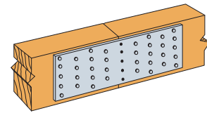
Typical TP39 installation (TP311 similar)
