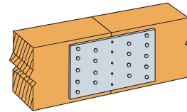
Typical TP35 installation (TP37 similar)
