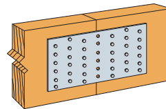
Typical TP47 installation
