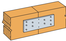
Typical TP15 installation
